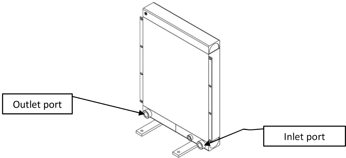
Sample of 2 pass cooler element.
